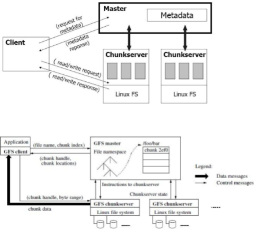
Figure 1: GFS Architecture
