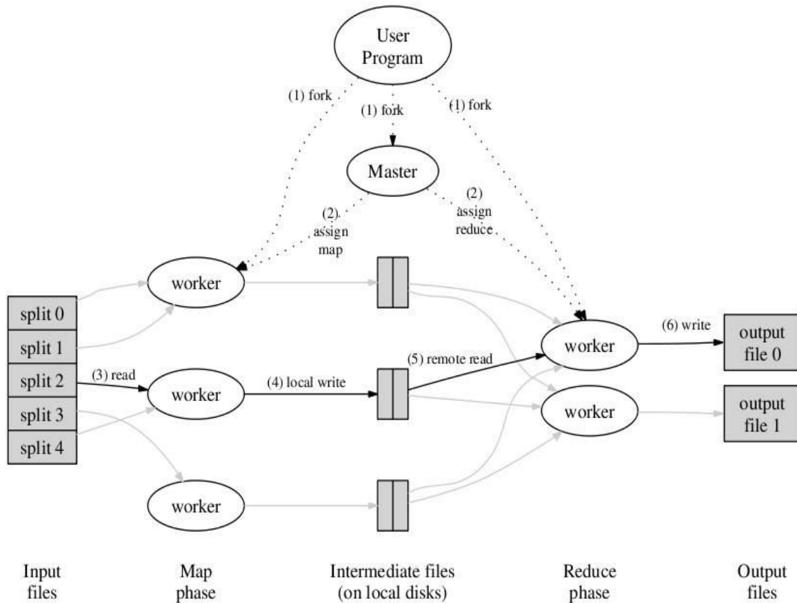
Figure 1: Execution overview
