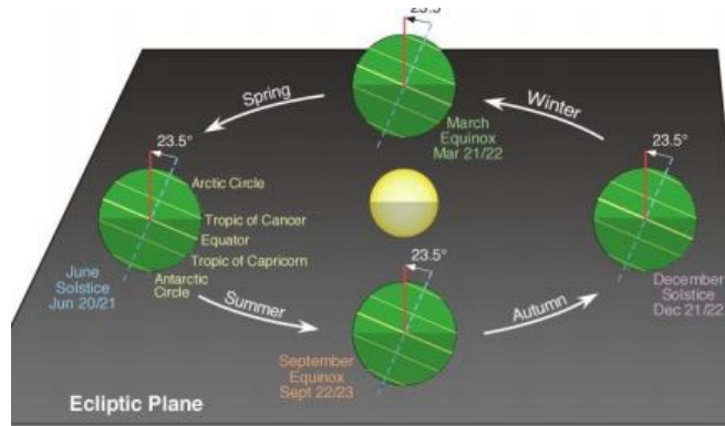
Figure 3.1.6: Movement of earth around sun.
