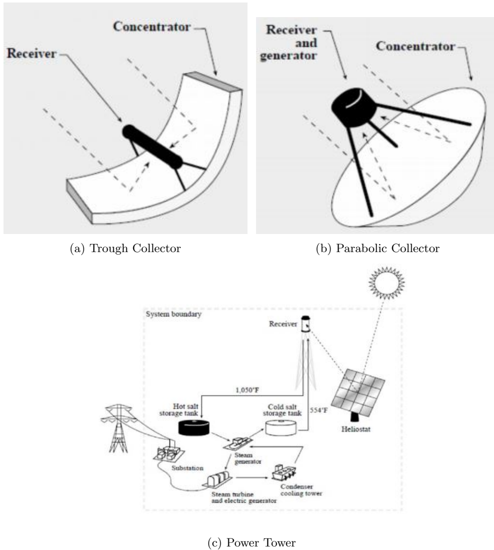
Figure 3.1.9: Concentrating collectors types.
