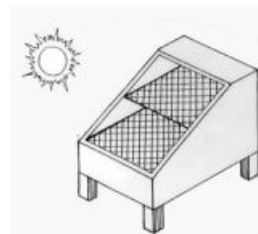
Figure 3.1.13: Cabinet solar drier.
