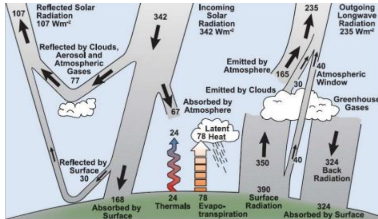
Figure 2.6.2: Radiation energy balance adopted by IPCC(2007).
