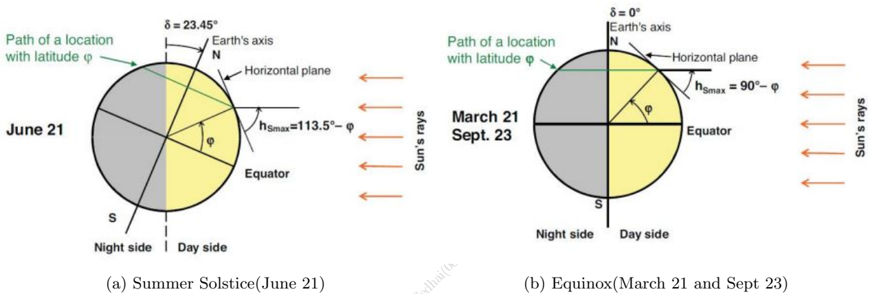
Figure 3.1.7: Summer solstice and equinox.
