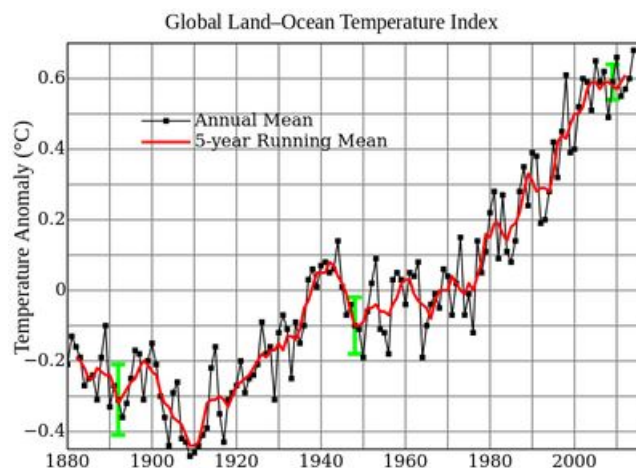
Figure 2.6.1: Temperature variation in earth.
