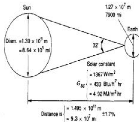
Figure 3.1.1: Sun and Earth.
