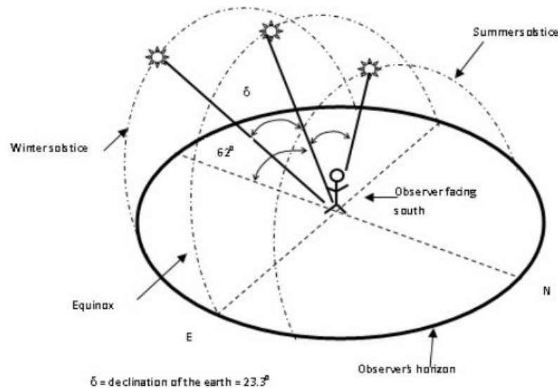
Figure 3.1.3: Apparent motion of Sun
