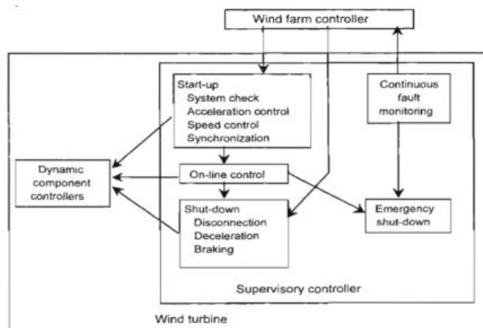
Figure 3.3.3: Wind turbine control systems.
