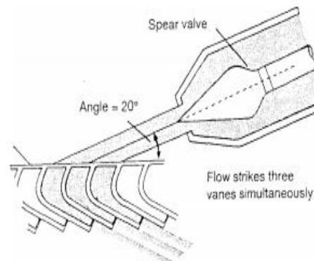
Figure 3.2.5: Turgo Turbine.
