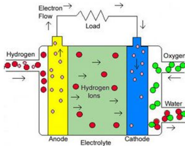
Figure 3.7.4: Phosphoric Acid
