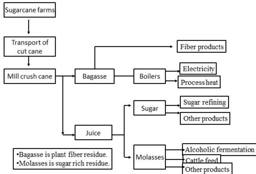
Figure 3.5.4: Biomass example: Sugarcane Agro Industry
