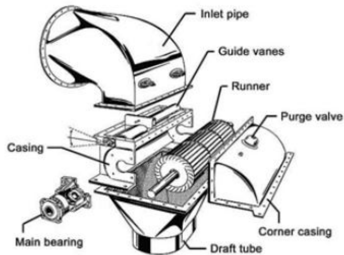
Figure 3.2.6: Crossflow Turbine.
