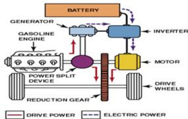
(c) Series parallel hybrid vehicles.
