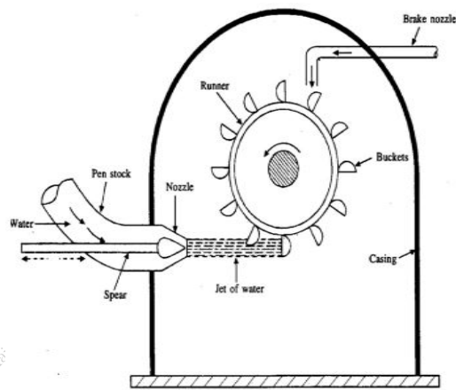
Figure 3.2.4: Pelton turbine.
