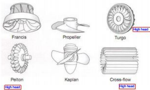
Figure 3.2.3: Types of turbine.
