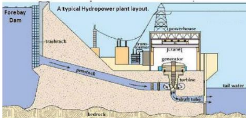
Figure 3.2.1: Hydropower general structure.
