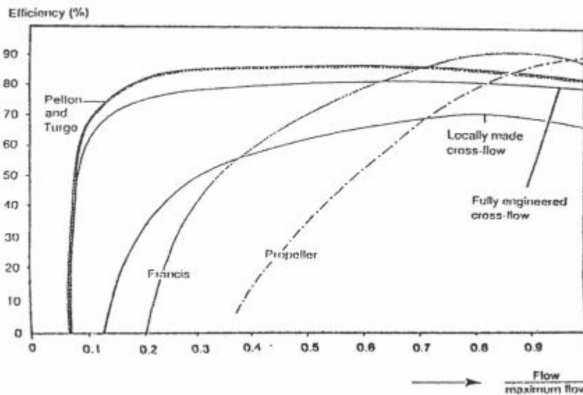
Figure 3.2.9: Turbine efficiency at different part flow conditions.
