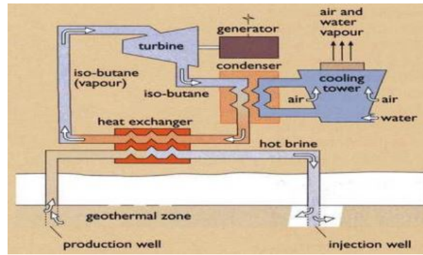
Figure 3.4.3: Binary cycle geothermal plant.
