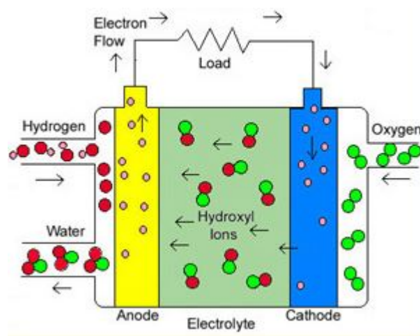
Figure 3.7.2: Alkali Fuel Cell
