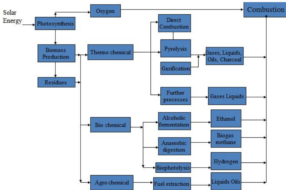
Figure 3.5.2: Biomass Conversion Process
