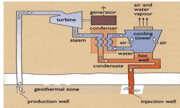
Figure 3.4.1: Dry steam geothermal plant.
