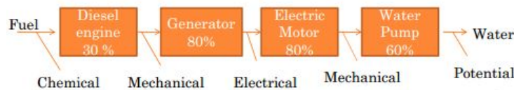
Figure 2.1.1: Effect of intermediate process while calculating efficiency.
