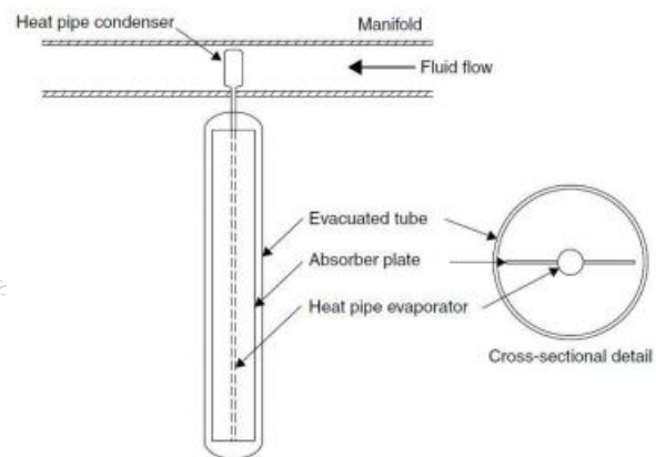
Figure 3.1.12: Evacuated tube flat plate Collector solar heater.
