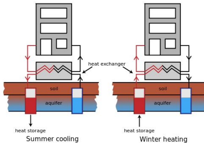
Figure 3.4.4: Geothermal heat pump during summer and winter.
