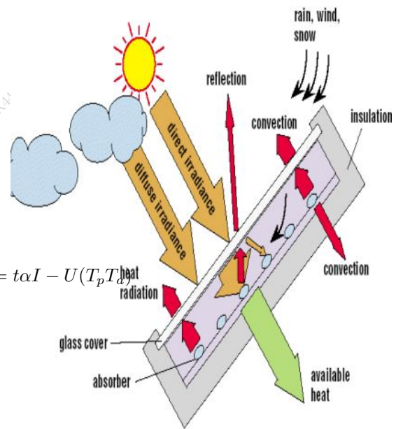
Figure 3.1.8: Flat plate collector.
