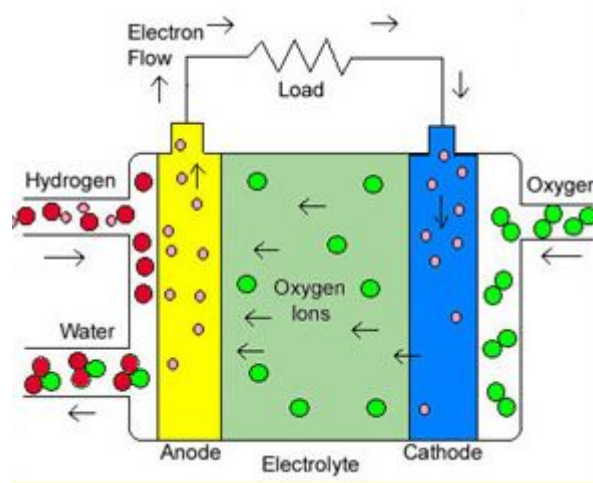
Figure 3.7.5: Solid Oxide
