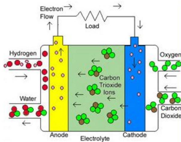
Figure 3.7.3: Molten Carbonate
