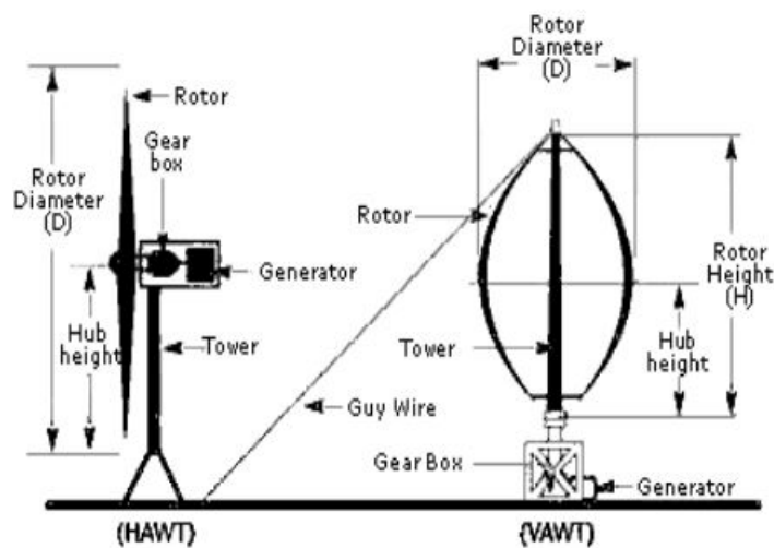
Figure 3.3.2: Types of wind turbines.
