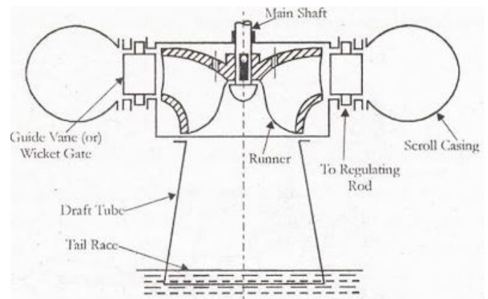
Figure 3.2.7: Francis Turbine.
