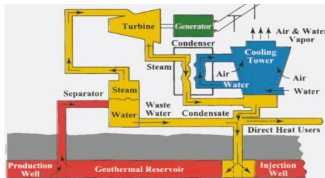
Figure 3.4.2: Flashed steam geothermal plant.
