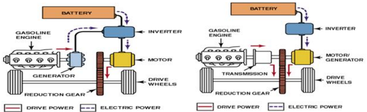
(a) Series hybrid vehicles.
