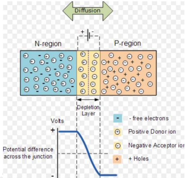
Figure 3.1.15: PN Junction.
