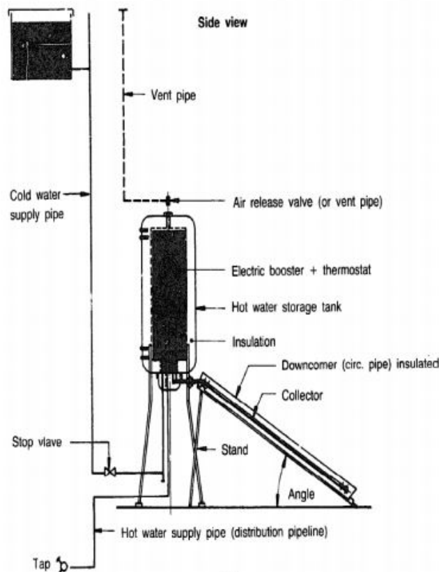
Figure 3.1.11: Thermosyphon solar water.
