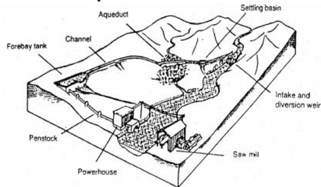
Figure 3.2.10: Major components of Micro Hydropower plant.
