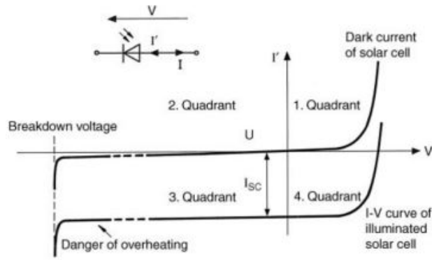
Figure 3.1.17: Solar cell, I-V characteristics.
