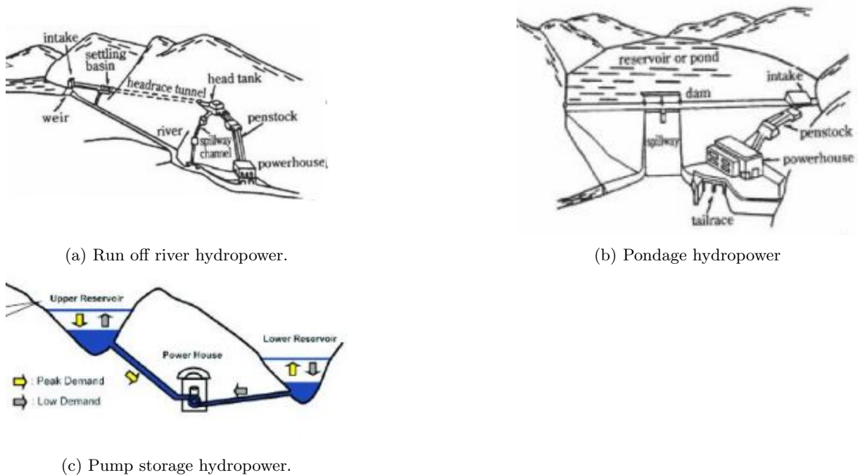
Figure 3.2.2: Hydropower types.
