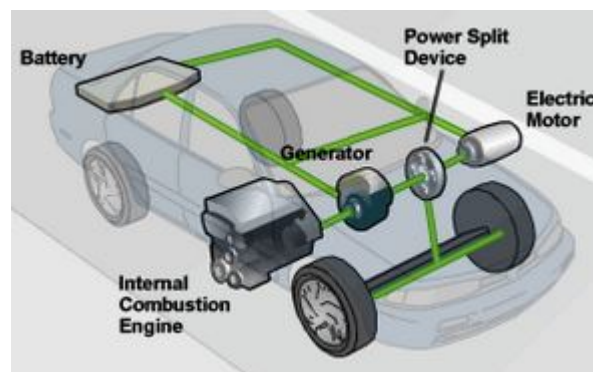
Figure 5.1.1: Hybrid vehicle having two source, petroleum and electricity.
