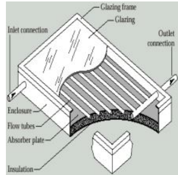
Figure 3.1.10: Solar water heater sectional view.
