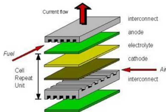
Figure 3.7.6: Planar Solid Oxide
