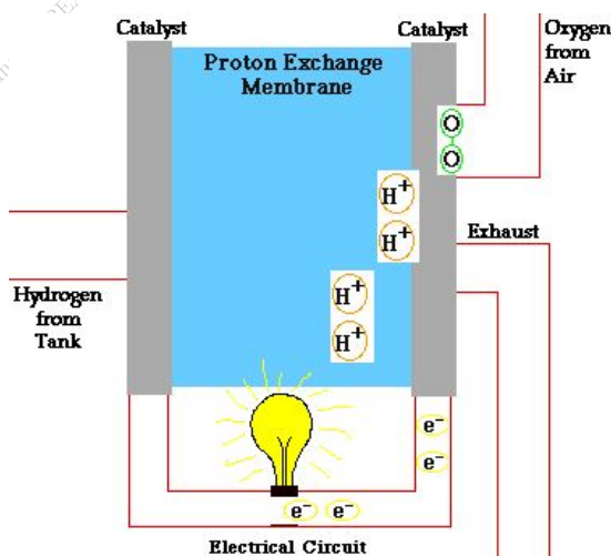
Figure 3.7.1: Fuel cell operations.
