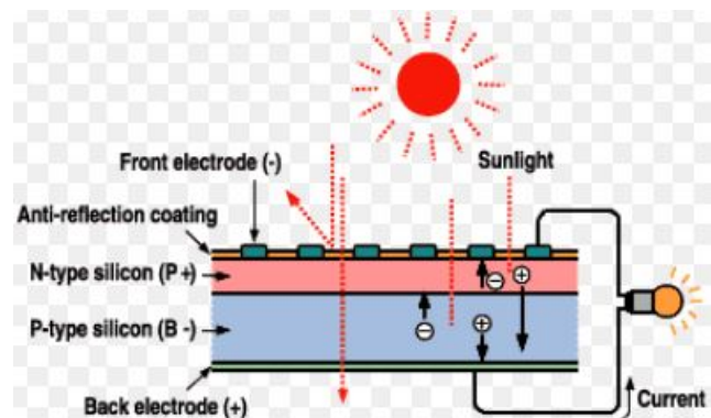
Figure 3.1.16: Solar cell structural section view.
