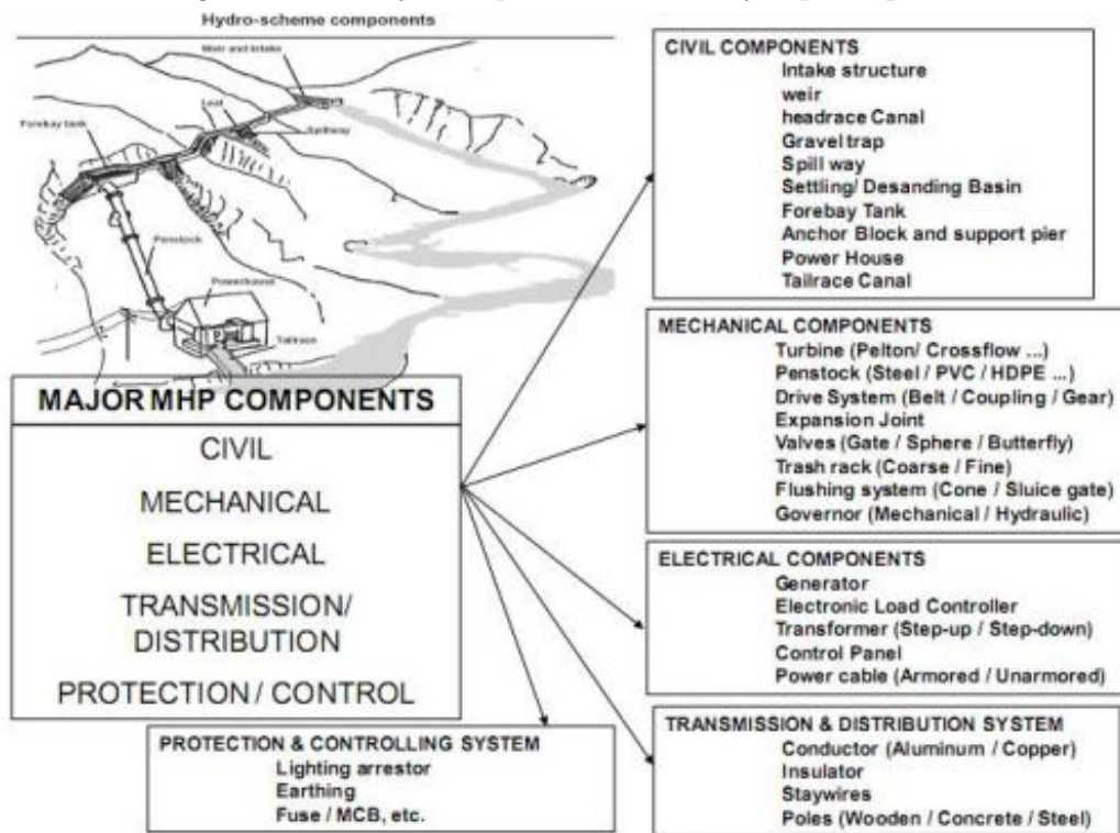
Figure 3.2.10: Major components of Micro Hydropower plant.
