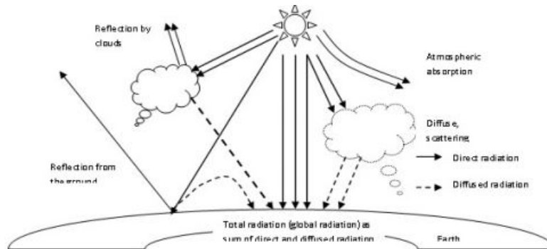
Figure 3.1.2: Arrival of solar energy on Earth .
