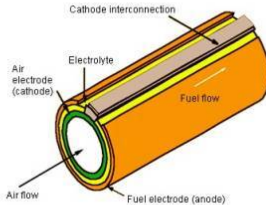
Figure 3.7.7: Tubular Solid Oxide
